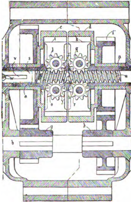
FIG. 357.—Longitudinal Section through the De Dion & Bouton Two-speed Change Gear.
